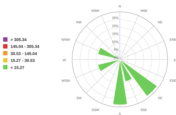
PM 100 (μg/m 3 )
