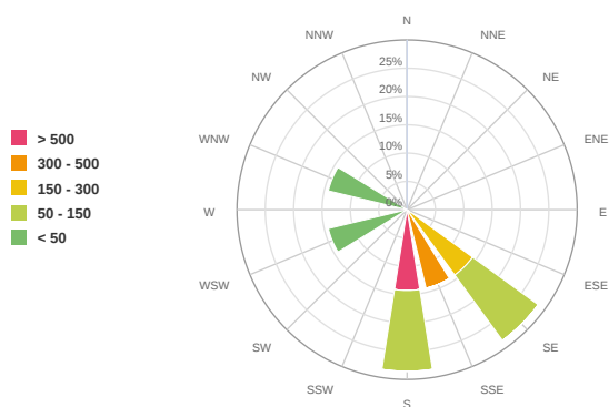
PM 100 (μg/m 3 )
