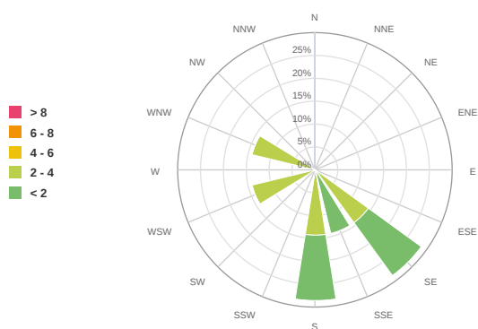
SO 2 (ppb)
