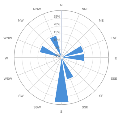
PM 1 (μg/m 3 )
