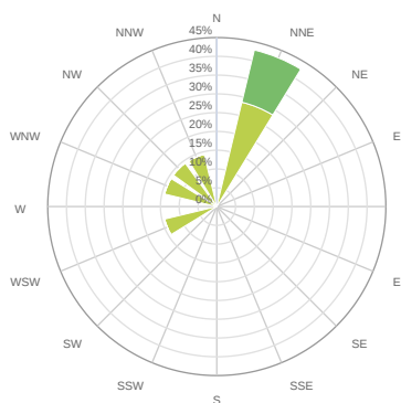
PM 100 (μg/m 3 )
