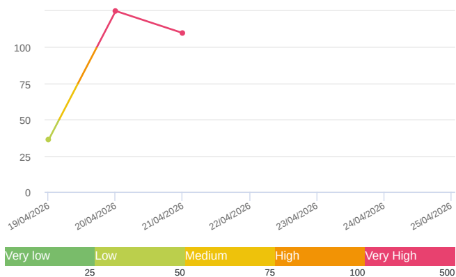
PM 2.5 (μg/m 3 )
