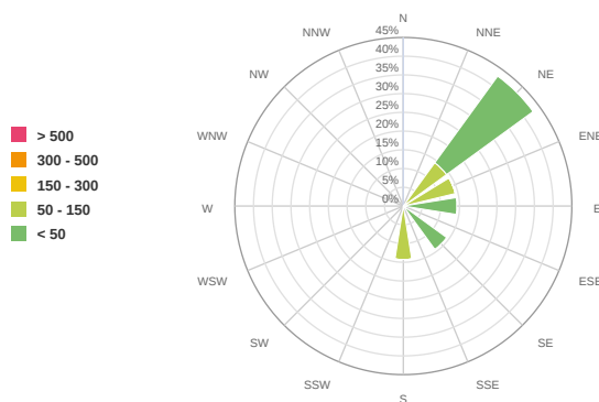
PM 100 (μg/m 3 )
