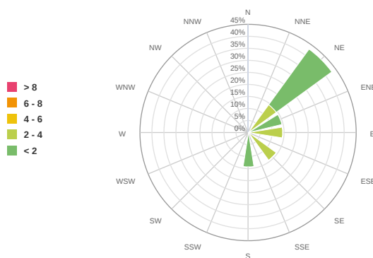
SO 2 (ppb)
