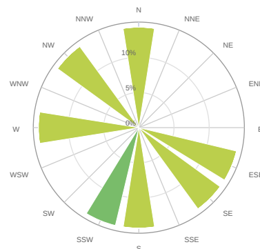
PM 100 (μg/m 3 )
