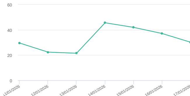
PM 2.5 (μg/m 3 )
