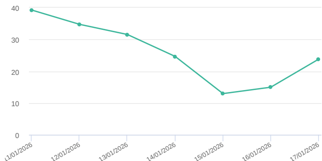
O 3 (μg/m 3 )
