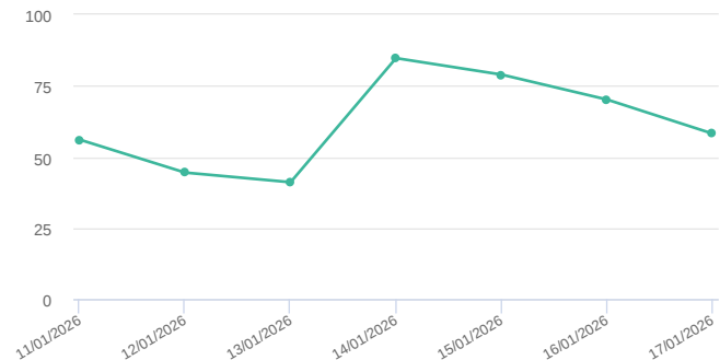
PM 10 (μg/m 3 )
