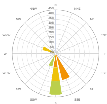
CO (ppb)
