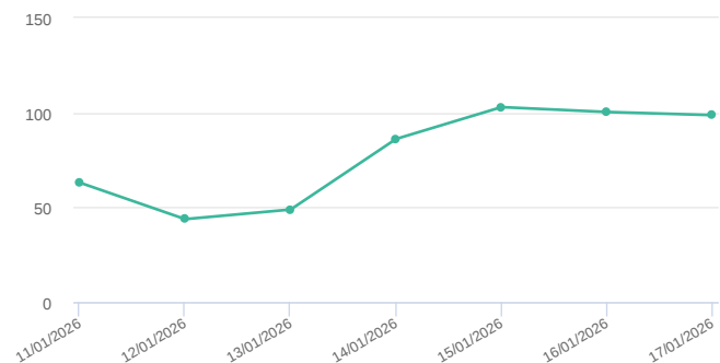
PM 10 (μg/m 3 )
