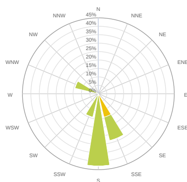
PM 100 (μg/m 3 )
