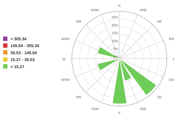
PM 100 (μg/m 3 )
