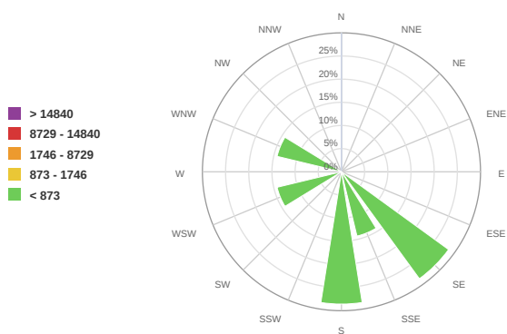
PM 1 (μg/m 3 )
